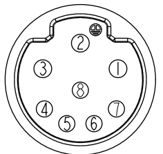
C1 Pin Assignments Front View
