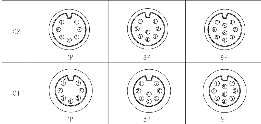
Pin Assignments Front View
