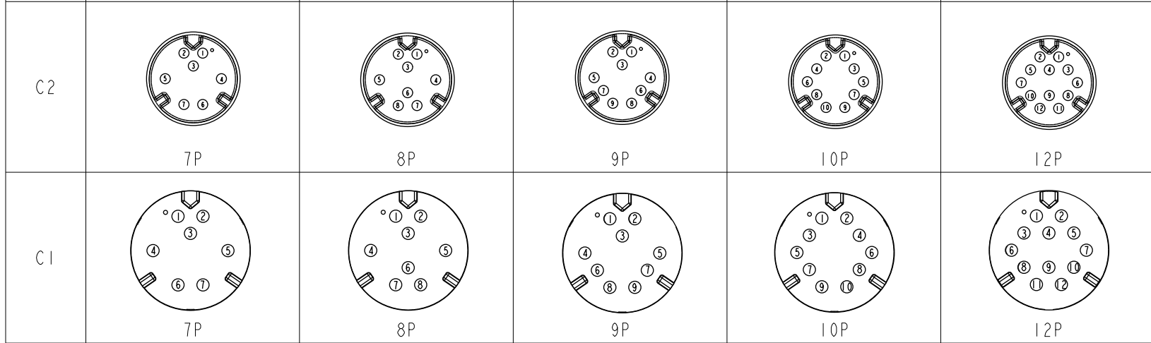
Pin Assignments Front View
