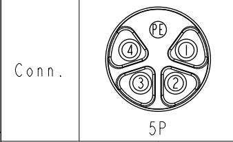
△B Pin Assignments Front View
