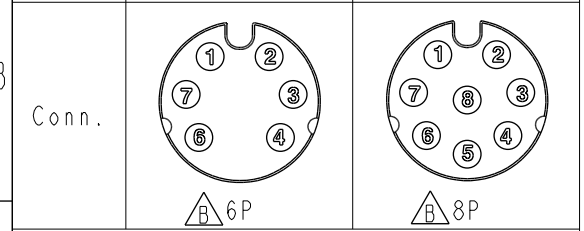
\triangle D Pin Assignments Front View
