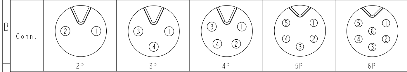
△B Pin Assignments Front View
