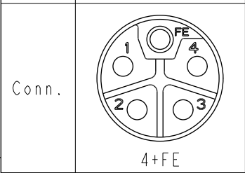
Pin Assignments Front View
