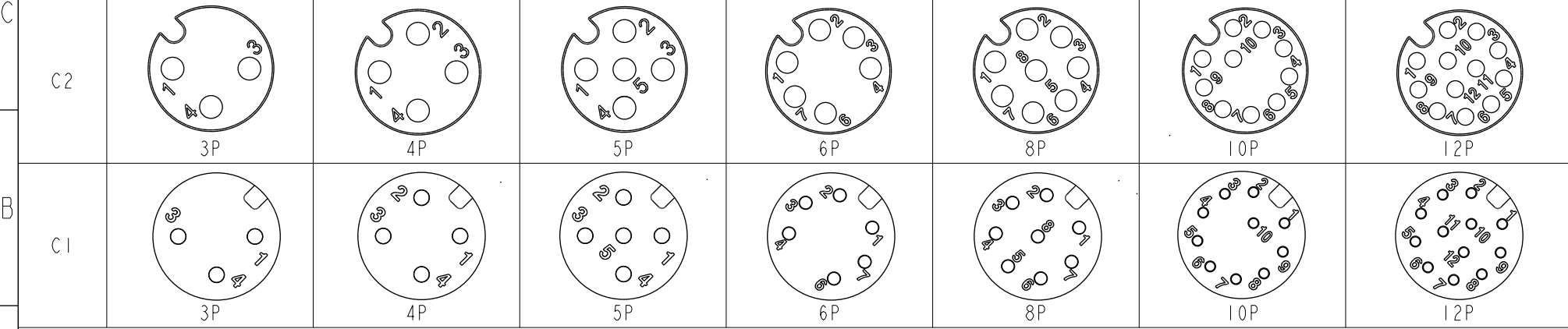
Pin Assignments Front View
