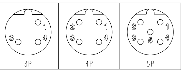
Pin Assignments Front View
