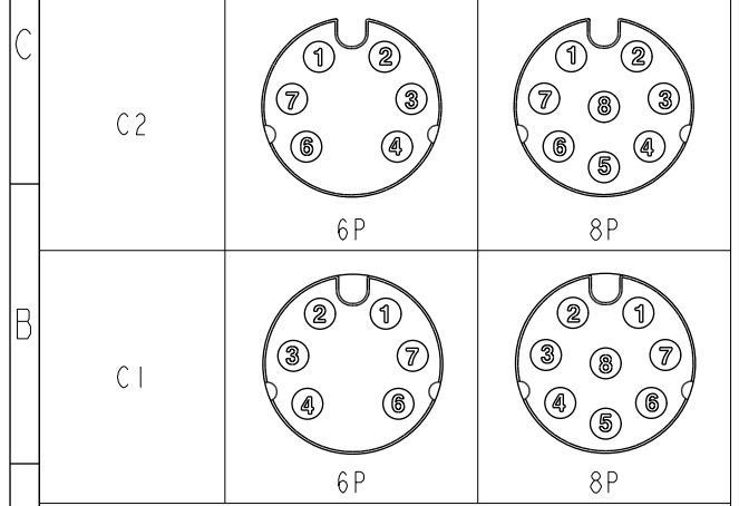
Pin Assignments Front View
