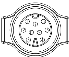
9Pin
