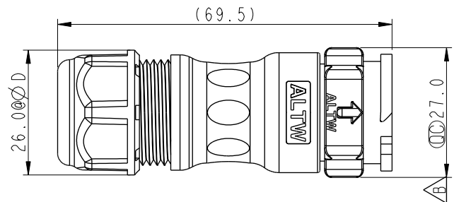
Sealing Nut
