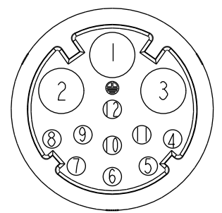
C1 Pin Assignments Front View
