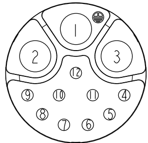
C1 Pin Assignments Front View
