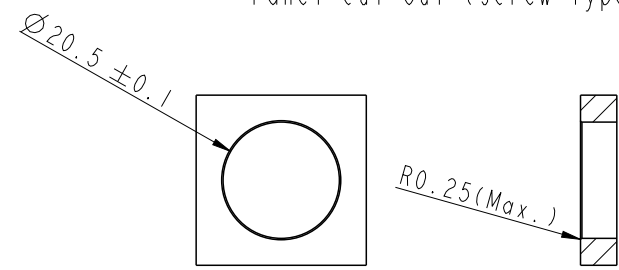
6.40 (Min.)/11.1 (Max.) Panel cut out (screw type)
