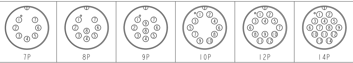
Pin Assignments Front View
