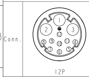
Pin Assignments Front View Pin Out
