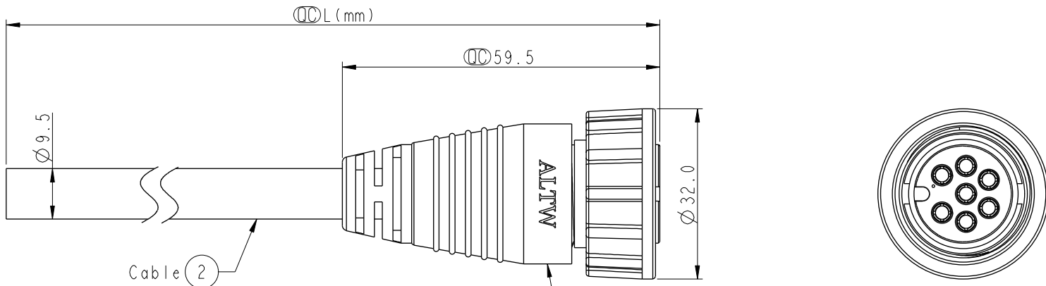
Conn.
